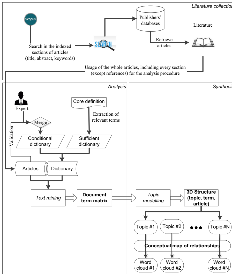
Fig. 1. Proposed approach.
